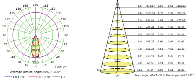
Luminous Intensity Distribution Curve
