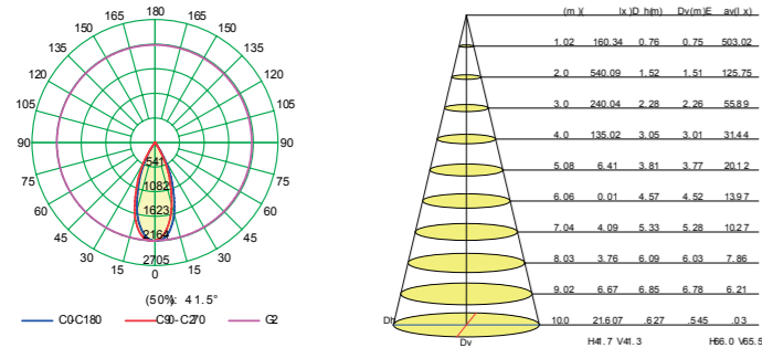
LED 15W 3000K 38°
