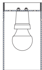
Sferic Bulb: Ø45*78
