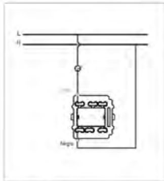
Interruptor Switch
