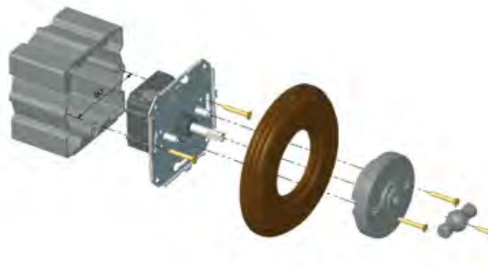
C Montaje de mecanismo Garby Colonial Assembling of Garby Colonial mechanism Montage du mécanisme Garby Colonial
